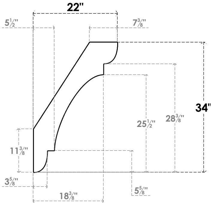
SIDE PROFILE
